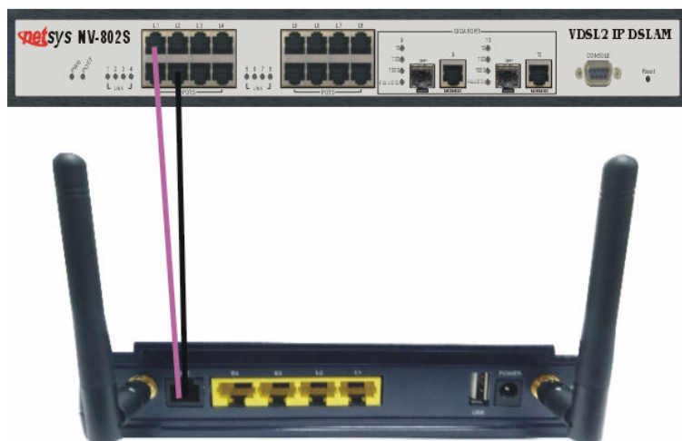
Figure 2.1 NV-720D line ports straight connection
