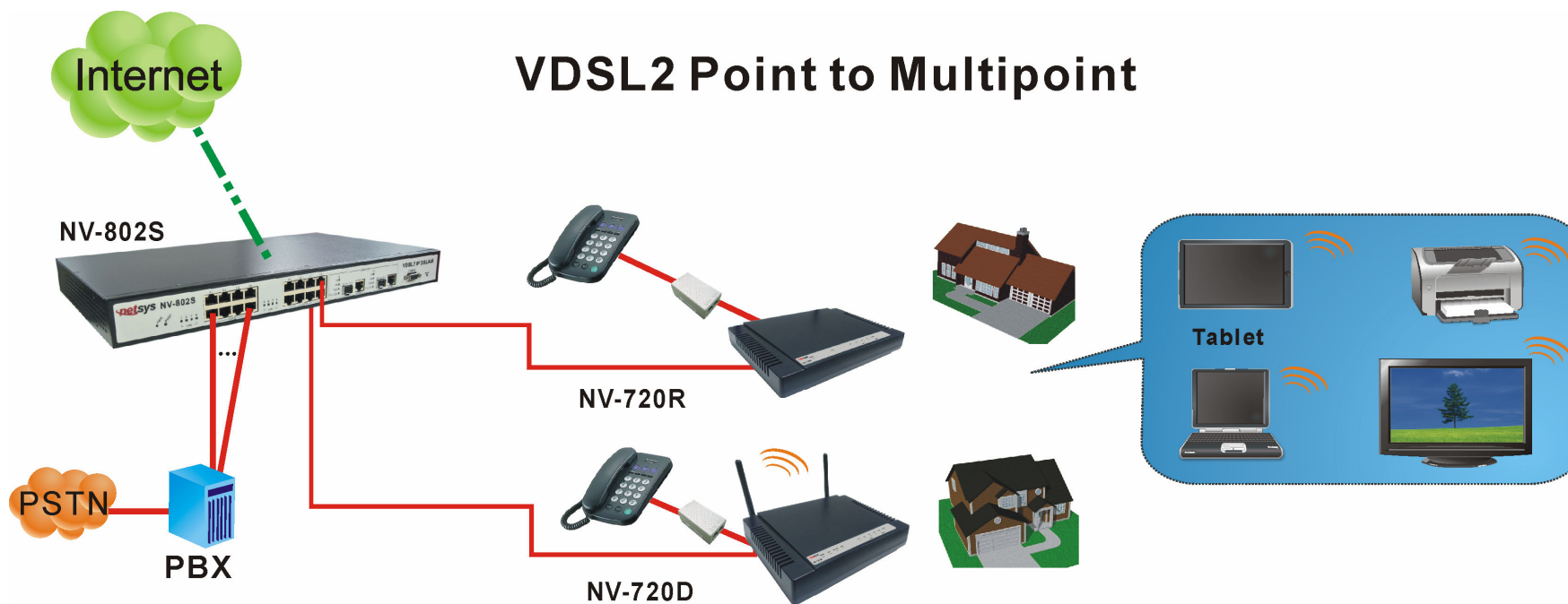
Figure 2.2.1 VDSL2 applications
