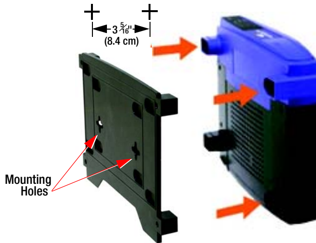
Figure 1: Wall Mounting
